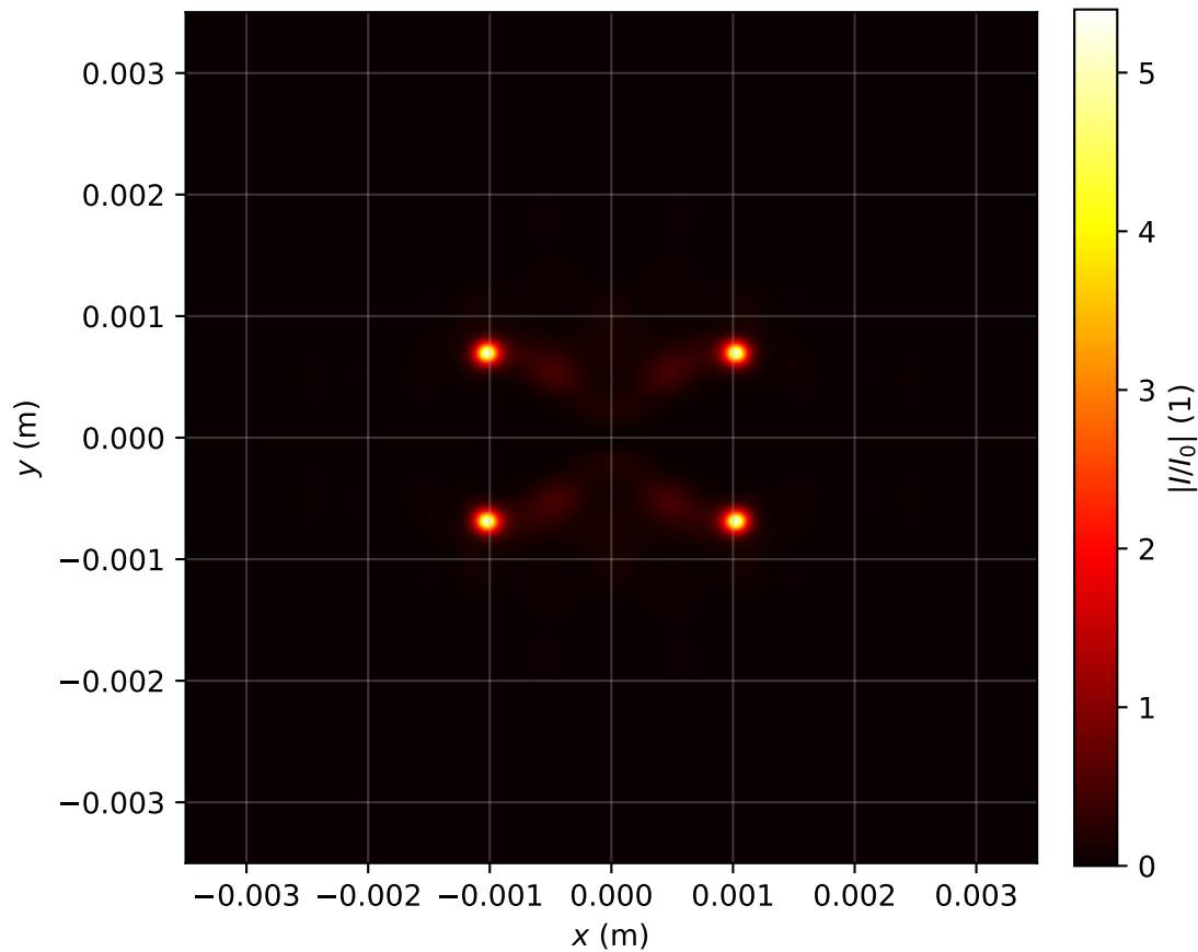
Intensity profile I(x, y, z = 1.751)/I_0 , P_{in}=9.0P_{cr} , artificial time
